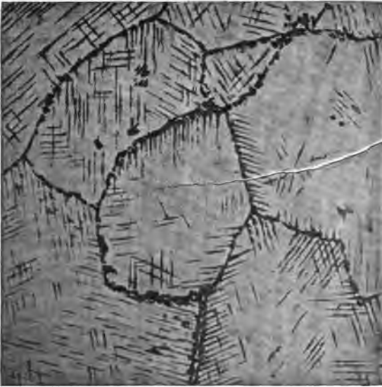
Fig. 1. Pearlite with Ferrite.
